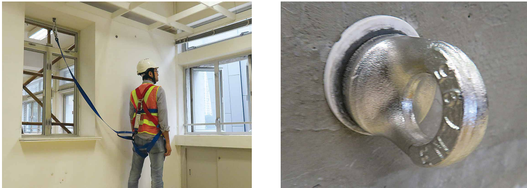
Figure 15: Full body safety harness attached to an independent anchorage
