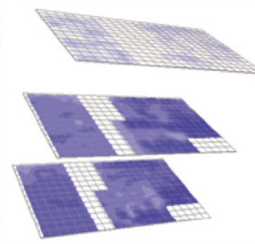
Microwave Tomography for Water Seepage Investigation
